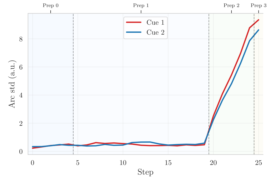
Arc-spacing std
