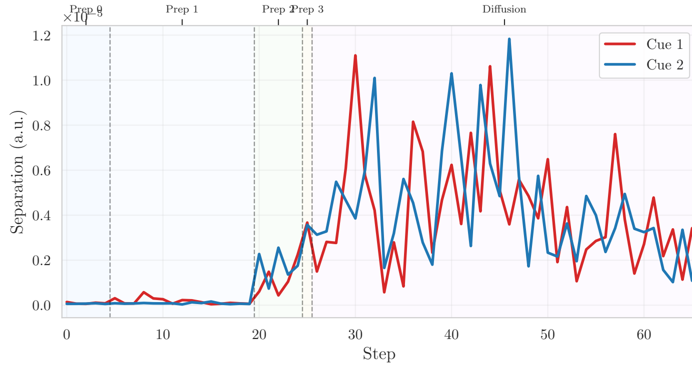
Centroid separation
