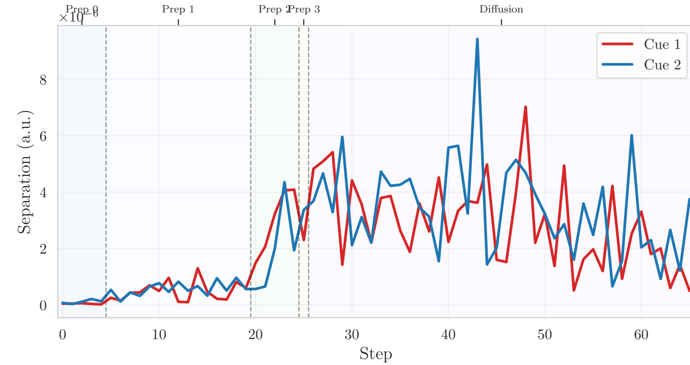
Centroid separation
