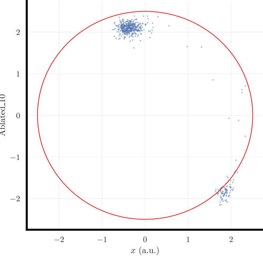
Generated samples
