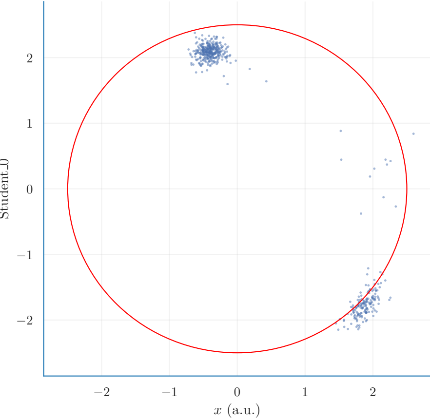
Samples overlay
