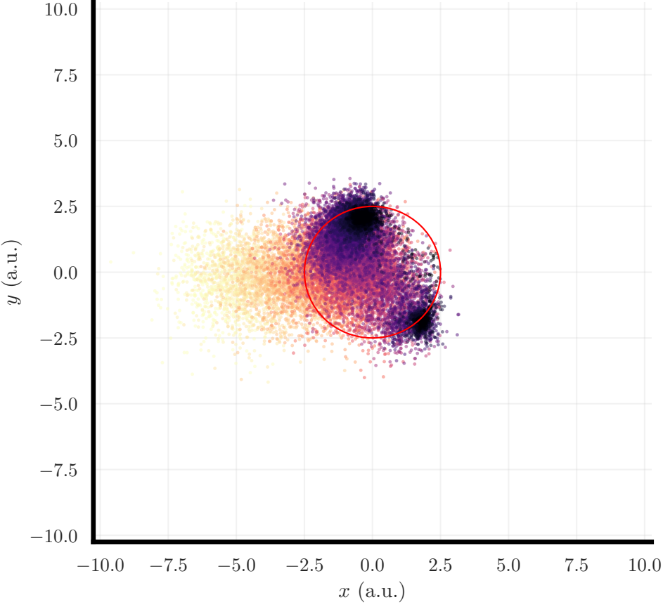
Sample trajectory
