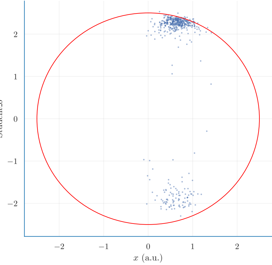
Samples overlay
