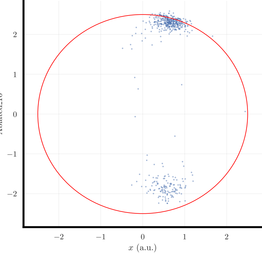
Generated samples
