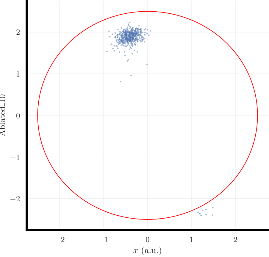
Generated samples
