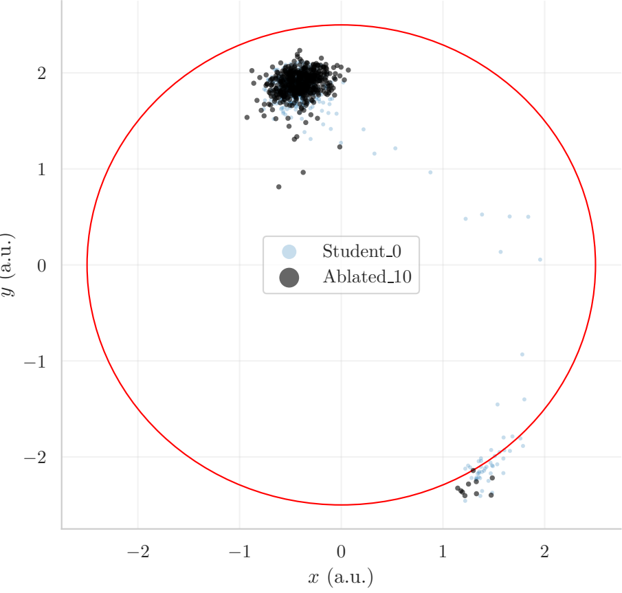
Samples overlay
