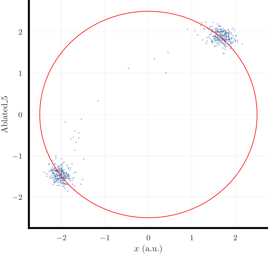
Generated samples
