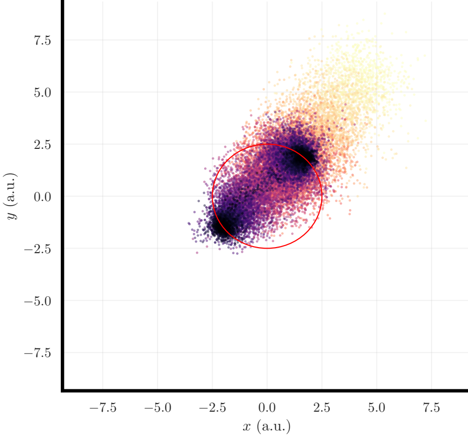
Sample trajectory
