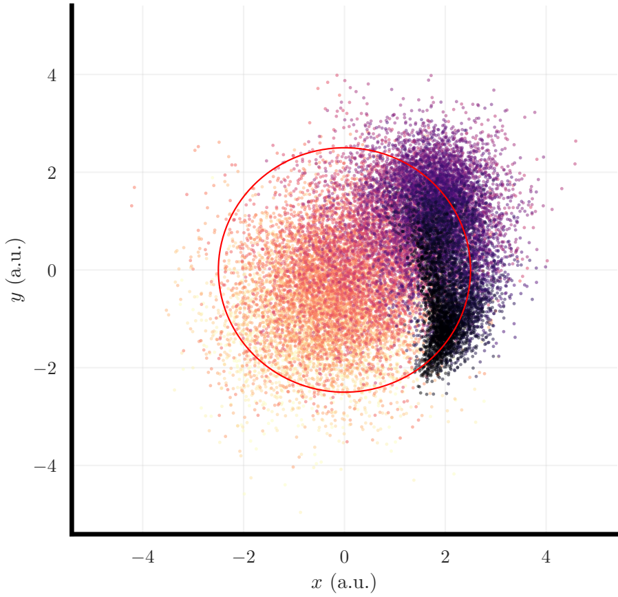
Sample trajectory
