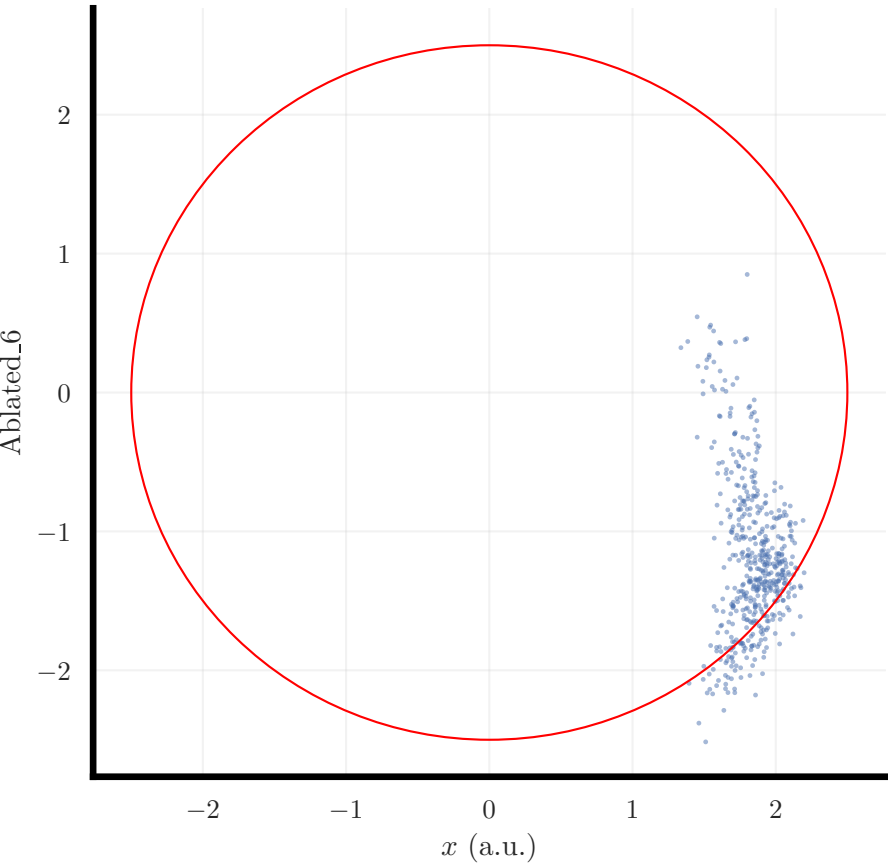
Generated samples
