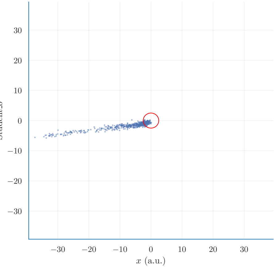
Samples overlay
