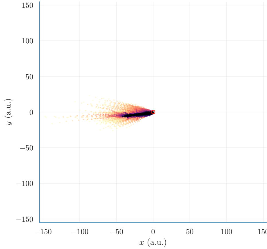
Sample trajectory
