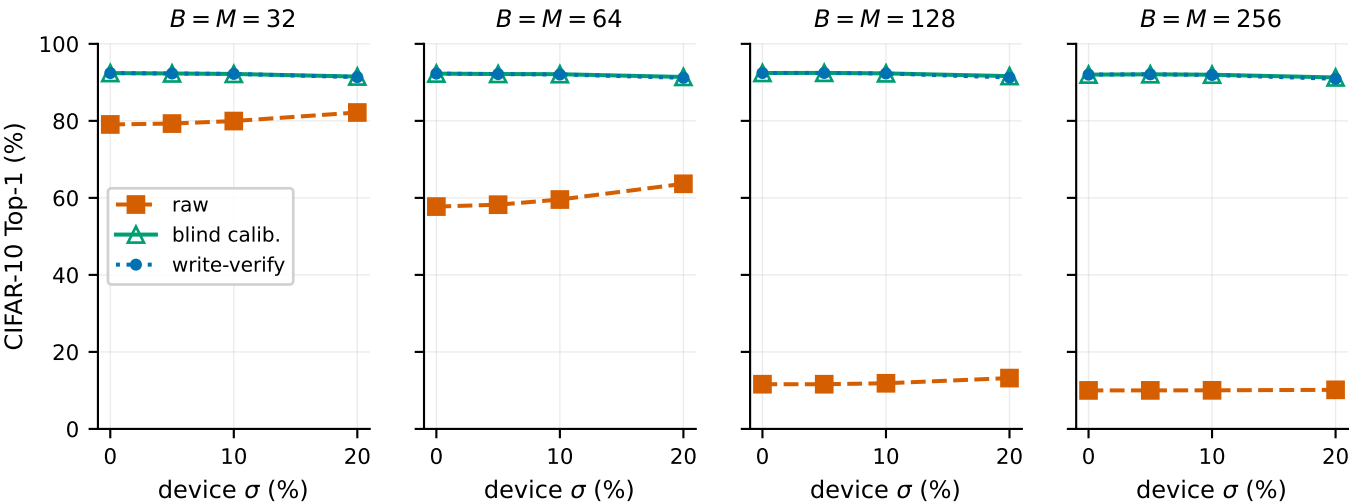
Gain calibration survives device variability at every tile height
