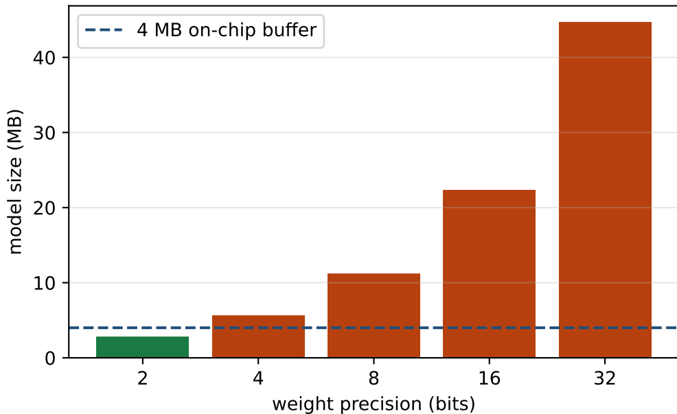
ResNet-18 fits a 4 MB buffer only at 2 bits or fewer
