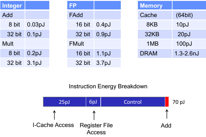
Figure 1.1.9: Rough energy costs for various operations in 45nm 0.9V.
