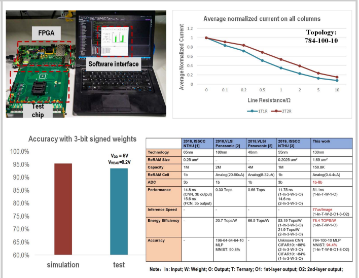
Figure 33.2.6: Test system and comparison table.
