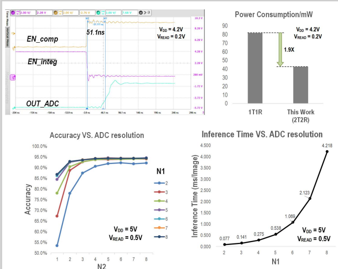
Figure 33.2.5: Measurement results during inference on MNIST dataset.
