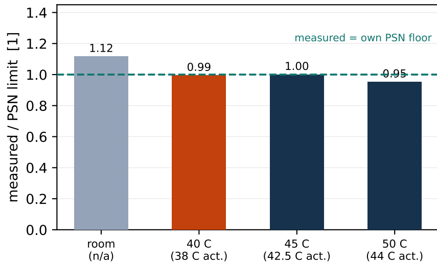
(b) no excess technical noise at any setpoint
