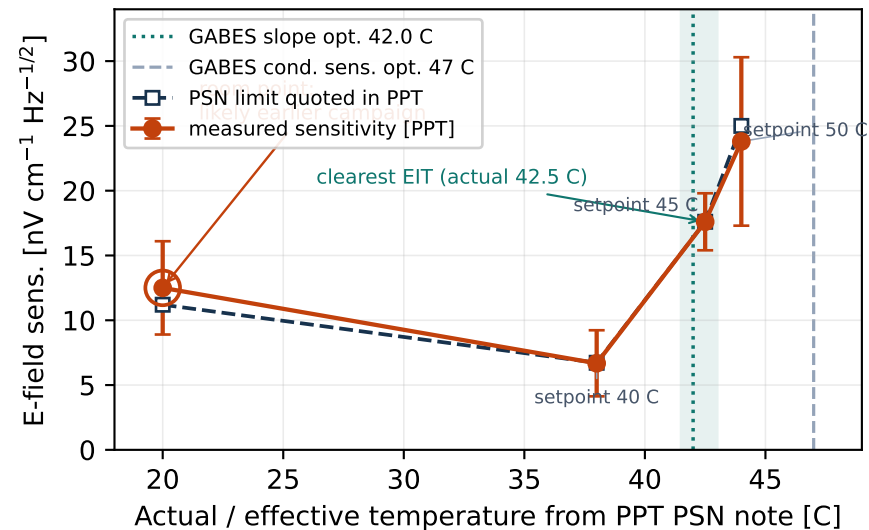
(a) sensitivity and its own PSN floor track each other
