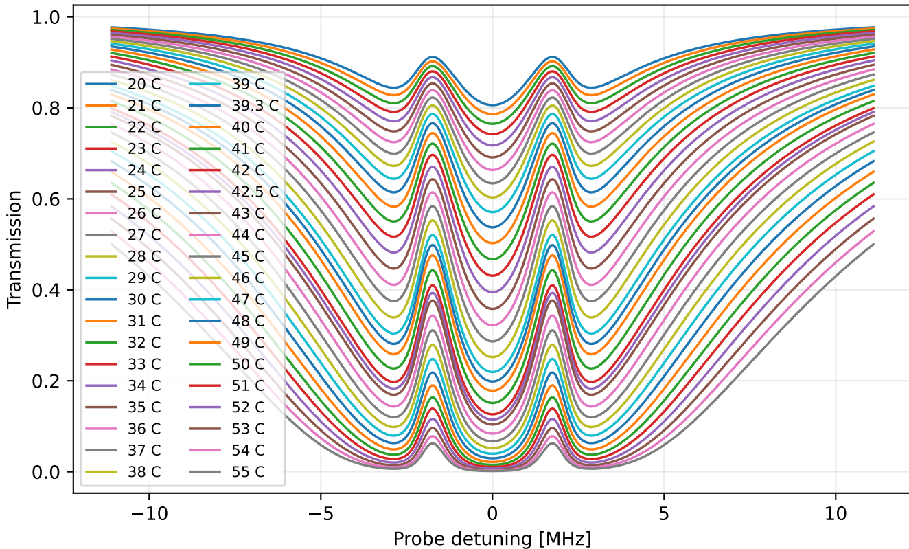
GABES AT electrometry: temperature sweep [PREDICTED]
