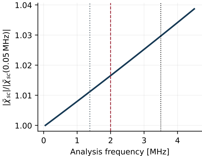
2-D Maxwell-averaged atomic response
