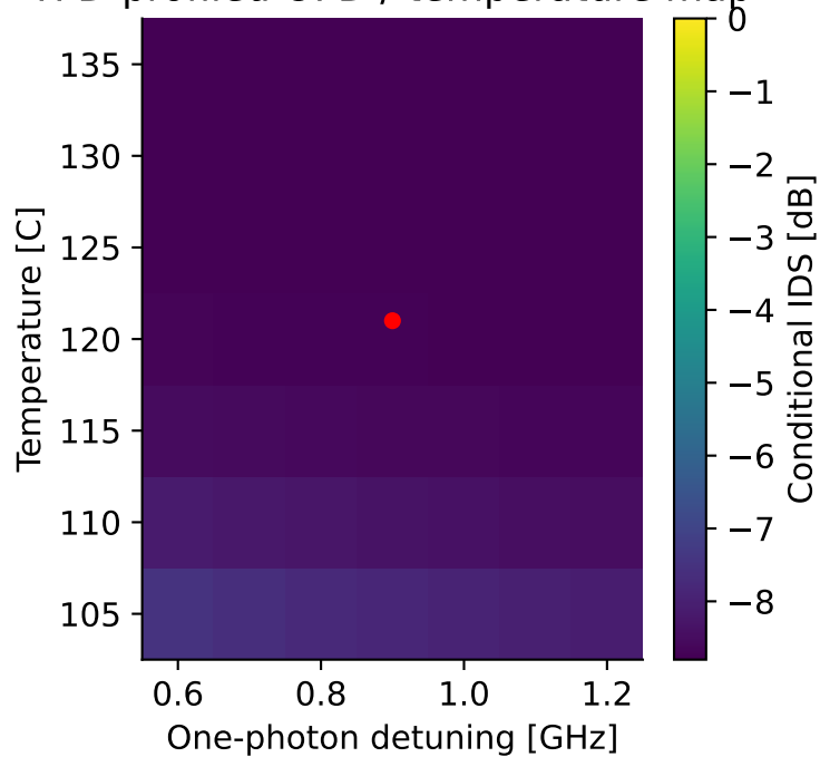
TPD-profiled OPD / temperature map
