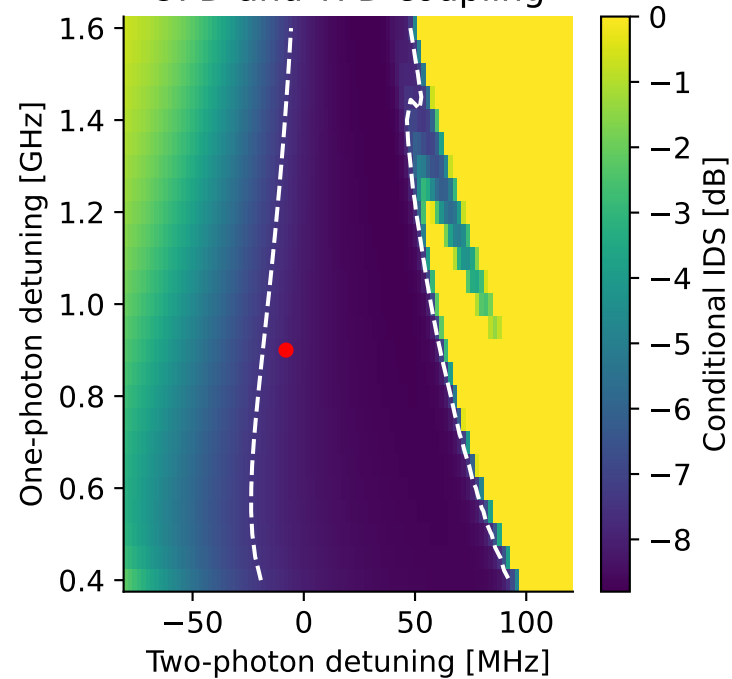
OPD and TPD coupling
