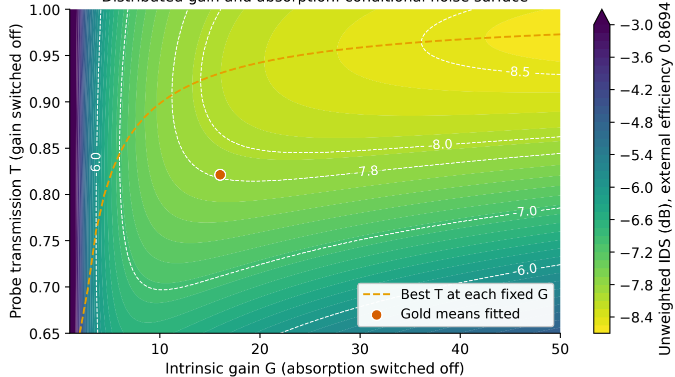
Distributed gain and absorption: conditional noise surface
