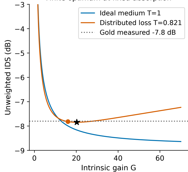
Finite optimum at fixed absorption
