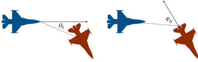
Fig. 3. Depiction of track angle \theta_t (left) and adverse angle \phi_a (right).
