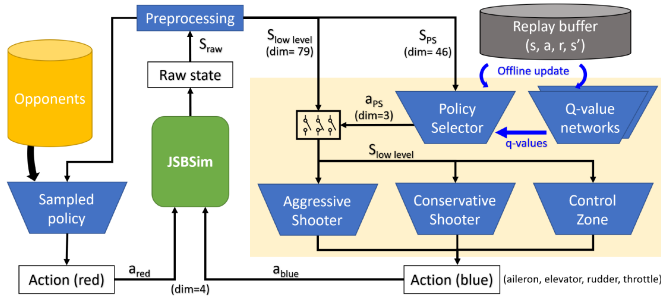
Fig. 7. Training architecture of the PHANG-MAN agent.
