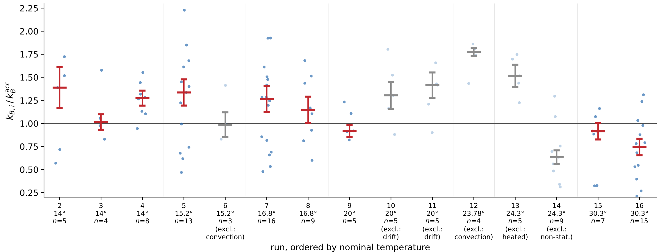
Per-bead k_B by run (bar: median \pm SE; line: accepted k_B , exact by SI definition)
