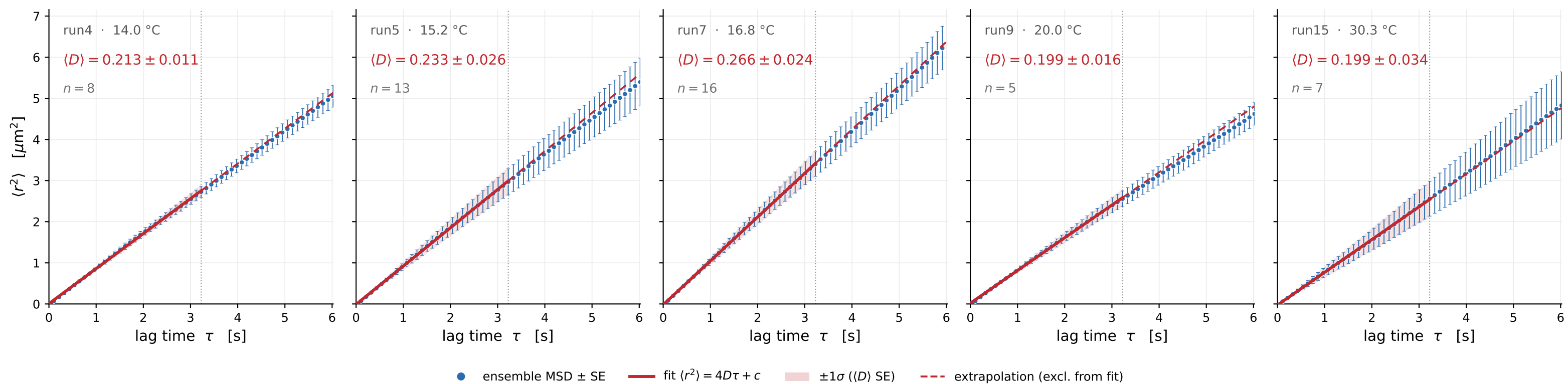
One representative run per temperature. Error bars = per-lag bead-to-bead SE ( \text{std}_{\text{beads}}/\sqrt{n} ; grows with \tau as different-radius beads diverge). \langle D \rangle \pm \text{SE} = ensemble-MSD fit over the SHORT-LAG window \tau \leq 3.2 s (band; free intercept c \approx 0 — localization \lesssim 1 px, so D is unbiased). Fig 2 k_B uses the per-bead median D , which agrees with \langle D \rangle to within 17%.
