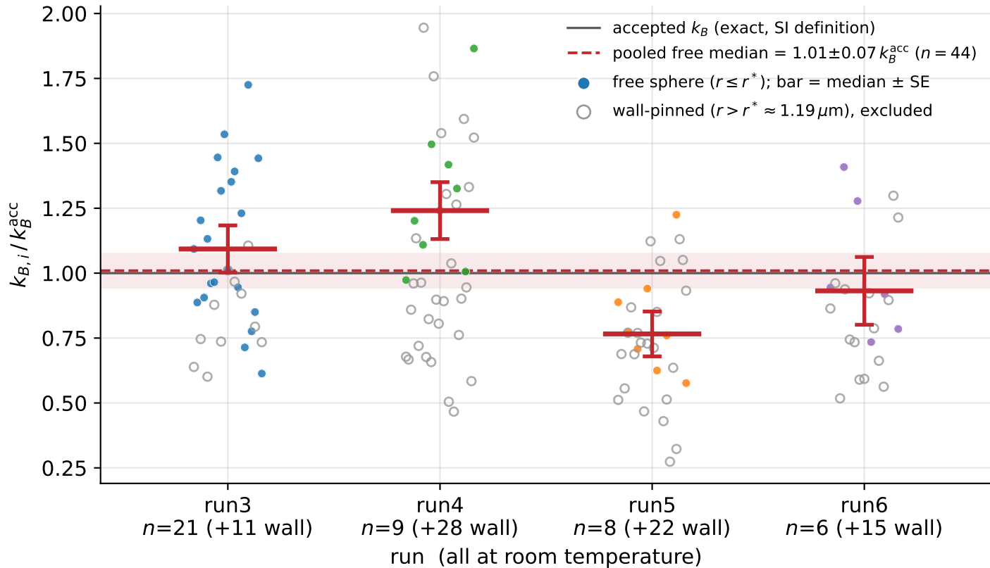
Week-1 per-bead k_B by run ( k_{B,i} = 6\pi\eta(T) r_i D_i / T ; free spheres r \leq r^* )
