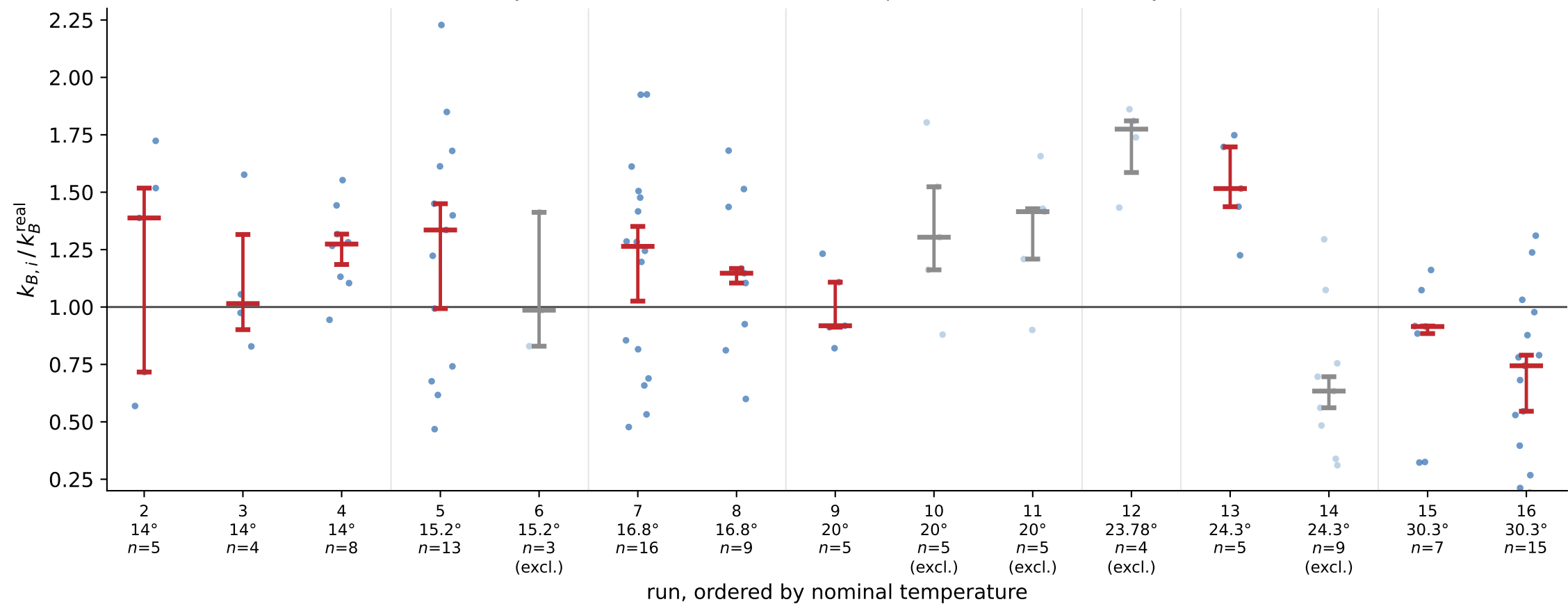
Per-bead k_B by run (bar: median \pm 68% bootstrap CI; line: real k_B , exact by SI definition)
