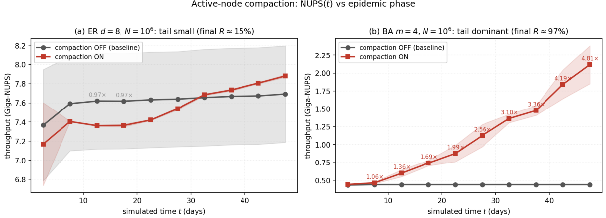
Figure 5: Active-node compaction: NUPS( t ) stratified into ten temporal windows of the TF = 50 renewal benchmark, 5 replicate trials (mean \pm 1 std shaded). Left: ER d=8 , N=10^6 , where the epidemic only reaches \approx 15\% attack rate within TF=50 ; compaction is \sim 3\% slower than baseline during the takeoff and peak windows (refresh overhead exceeds marginal skip gain) and crosses over to a small lift only in the last temporal bucket. Right: BA m=4 , N=10^6 , where explosive hub-driven takeoff reaches \approx 97\% attack rate; the shrinking active set drives a progressive speedup from 1.0\times (takeoff) to 4.8\times (last bucket, \text{num\_active} \approx 3\%N ), giving 1.53\times on the whole-run mean (Table 3). The topology-dependent pattern makes compaction a high-saturation / long-horizon optimisation: it is most valuable on scale-free networks, policy evaluations that simulate past the peak, and reinforcement-learning rollouts that run to extinction.
