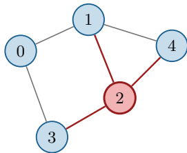
contact graph
