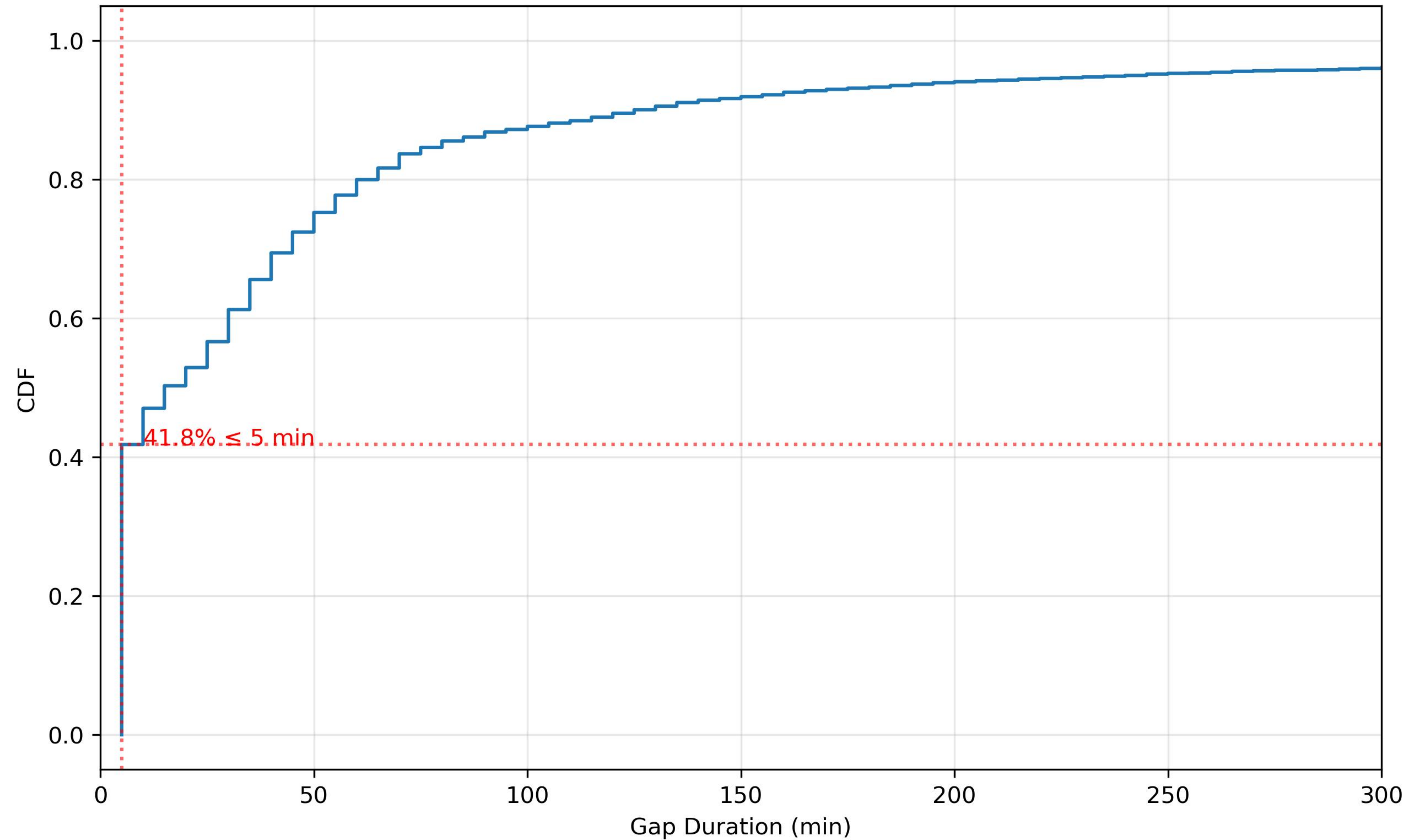
Night - Gap Duration CDF
