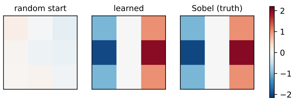
Figure 8.1.: The mystery-detector game. Left: the random starting kernel. Middle: the kernel after 600 steps of gradient descent on input–output pairs alone. Right: the hand-crafted vertical Sobel detector from Chapter 7’s zoo. Nobody told the middle panel what an edge is.
