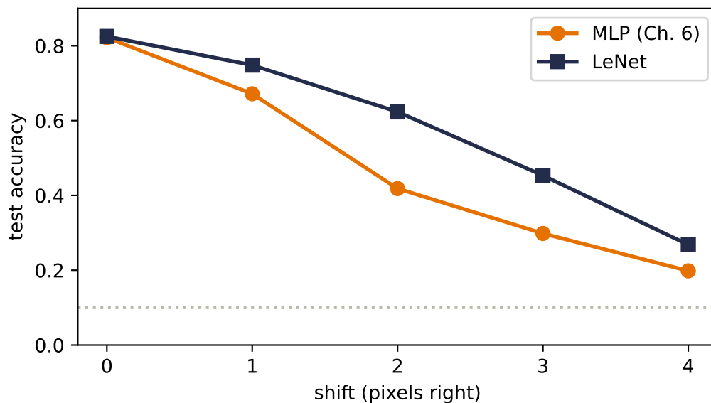
Figure 8.3.: The rematch. Chapter 6’s experiment, run on both architectures trained under the identical recipe. The MLP repeats its cliff: half its accuracy gone by two pixels. LeNet degrades gracefully — the same two-pixel shift costs it a quarter. The dotted line is chance.
