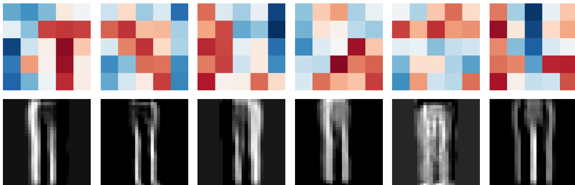
Figure 8.4.: What LeNet learned to look for. Top: the six first-layer 5 \times 5 kernels (red positive, blue negative). Bottom: each kernel's feature map on a test trouser — different detectives report left leg edges, right edges, interior fill. Trained on only 1,200 images the kernels are grainier than their full-dataset cousins, but the division of labor is unmistakable. Compare Chapter 6's full-frame templates: same job, opposite philosophy.
