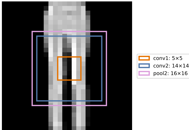
Figure 8.2.: What one neuron sees, by depth. Boxes mark the receptive field of a single unit in each stage of our network, centered on the same spot: conv1 sees a 5 \times 5 patch, conv2 sees 14 \times 14 , the final pooled cell 16 \times 16 . Local wiring, increasingly global sight; the dense head then reads all 25 such overlapping views at once.
