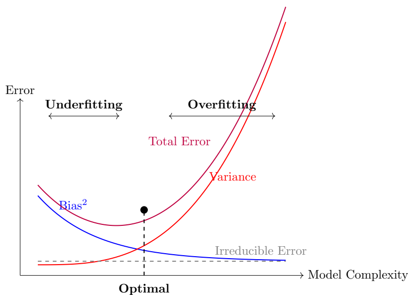
Figure 1.5.: The classical picture: as model complexity grows, bias falls while variance rises; total error is U-shaped, with sweet spots between under- and overfitting.
