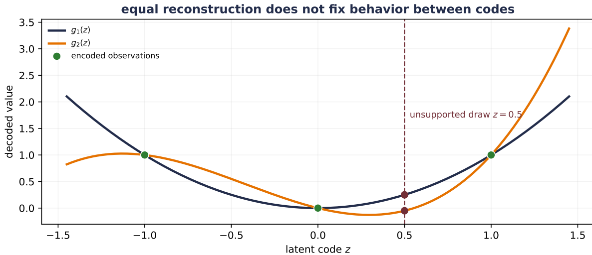
Figure 9.7.: Reconstruction does not identify a latent sampler or a unique decoder away from observed codes. The two displayed decoders agree exactly at z equal to -1 , 0 , and 1 , so both have zero reconstruction error on the three targets. They disagree between and beyond those codes; at z = 0.5 their outputs are 0.25 and -0.05 .
