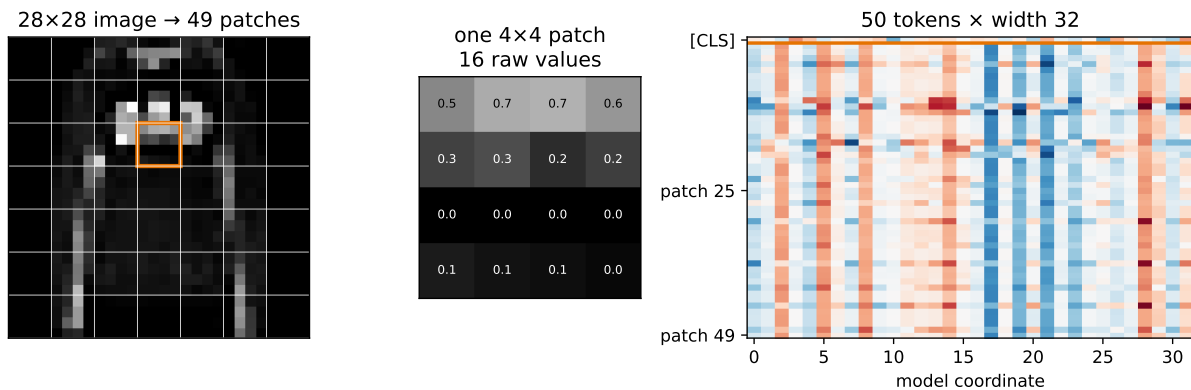
Figure 16.1.: An image becomes a sequence. A 28 \times 28 garment is divided into 49 nonoverlapping 4 \times 4 patches (left); one patch contains 16 raw values (center); a shared linear projection maps every patch to width 32, and a separate learned [CLS] row is prepended (right). The displayed projection is random arithmetic, not a trained representation.
