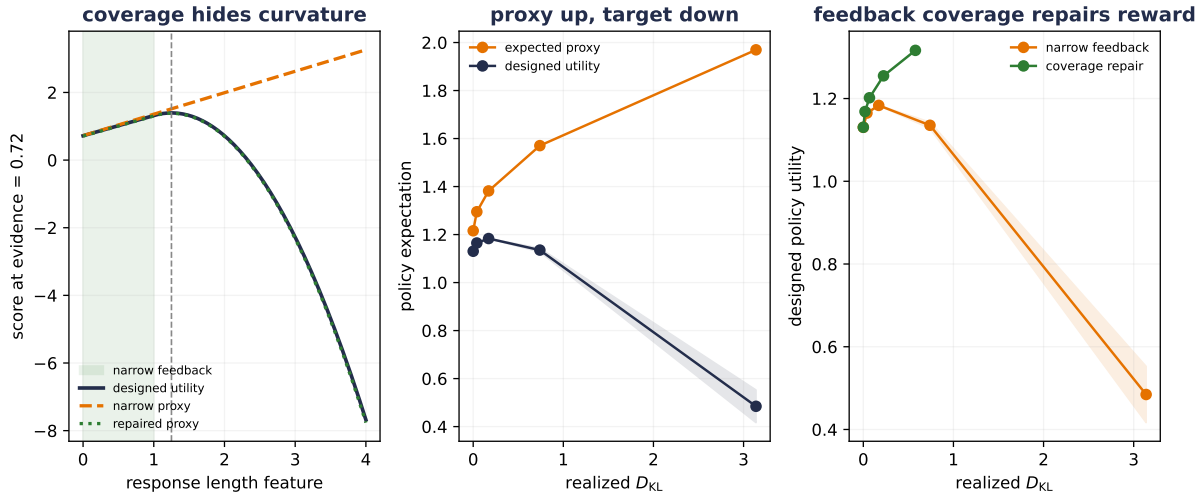
Figure 18.5.: A reward model can pass an in-range comparison test and fail under optimization.
