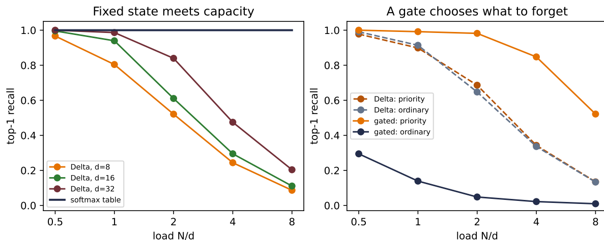
Figure 14.7.: A sealed synthetic mechanism test, not a language-model or state-space benchmark.
