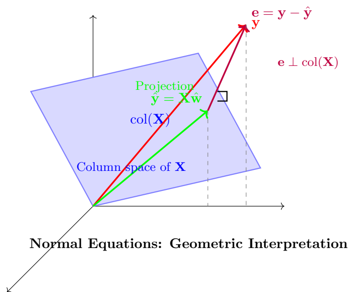
Figure A.1.: Projection separates what the columns can express from what they cannot. The fitted vector \hat{\mathbf{y}} lies in the column space; the residual is orthogonal to every column direction. The diagram labels that residual \mathbf{e} = \mathbf{y} - \hat{\mathbf{y}} ; the appendix uses \mathbf{r} for the same quantity.
