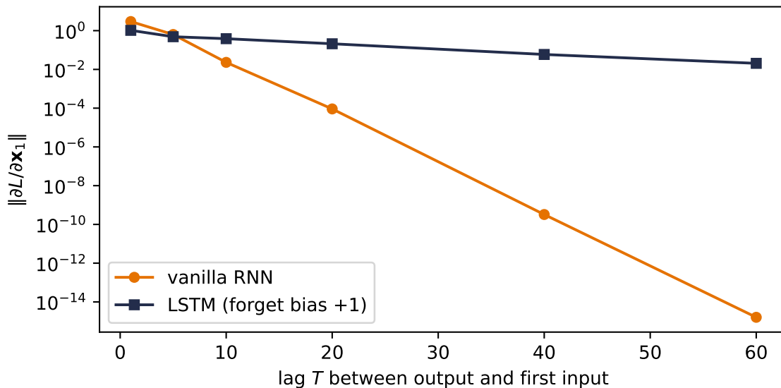
Figure 10.2.: The gradient-vs-lag experiment, rerun with an LSTM whose forget-gate bias is initialized to +1. The vanilla RNN’s blame signal dies its exponential death; the LSTM’s rides the cell-state conveyor belt and arrives at lag 60 attenuated but alive — thirteen orders of magnitude stronger. Chapter 9 built this highway across layers; the LSTM builds it across time, with a learned valve on the on-ramp.
