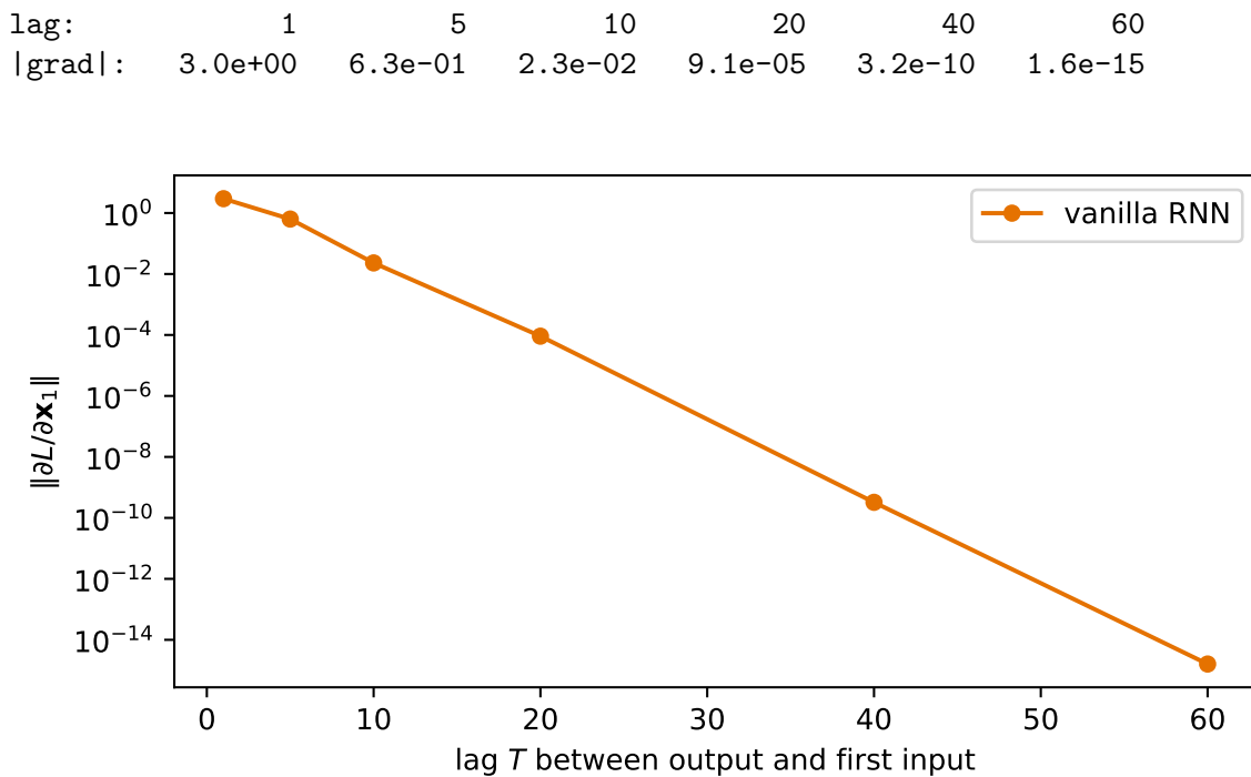
Figure 10.1.: How much a freshly initialized vanilla RNN’s output can blame its first input, as the lag between them grows. Fifteen orders of magnitude gone by sixty steps: the same exponential decay Chapter 5 measured down a deep network, now measured across time — because an unrolled RNN is a deep network with tied weights.
