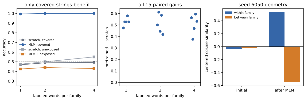
Figure 15.5.: Five paired end-to-end seeds in the synthetic transfer lab. MLM initialization separates covered latent families and improves every covered-type comparison (left and center); both arms stay near chance on input-vocabulary controls withheld from MLM inputs, replacements, and targets (left). Centered cosine similarity is a representation diagnostic, not a task metric (right).
