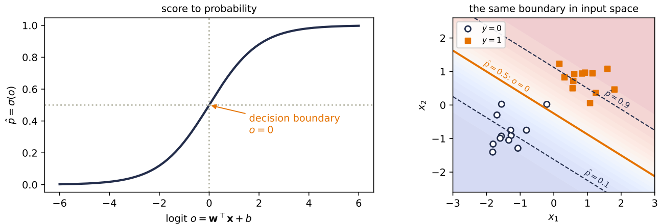
Figure 2.1.: The sigmoid maps any real score to (0, 1) , crossing \frac{1}{2} exactly at o = 0 (left). In input space (right), that single score is the straight line \mathbf{w}^\top \mathbf{x} + b = 0 between the circles and the squares; the dashed contours \hat{p} = 0.1 and 0.9 are parallel to it. Confidence grows with distance from the line, and the line itself never bends. The model’s uncertainty lives near the boundary; its confident regions saturate far from it.
