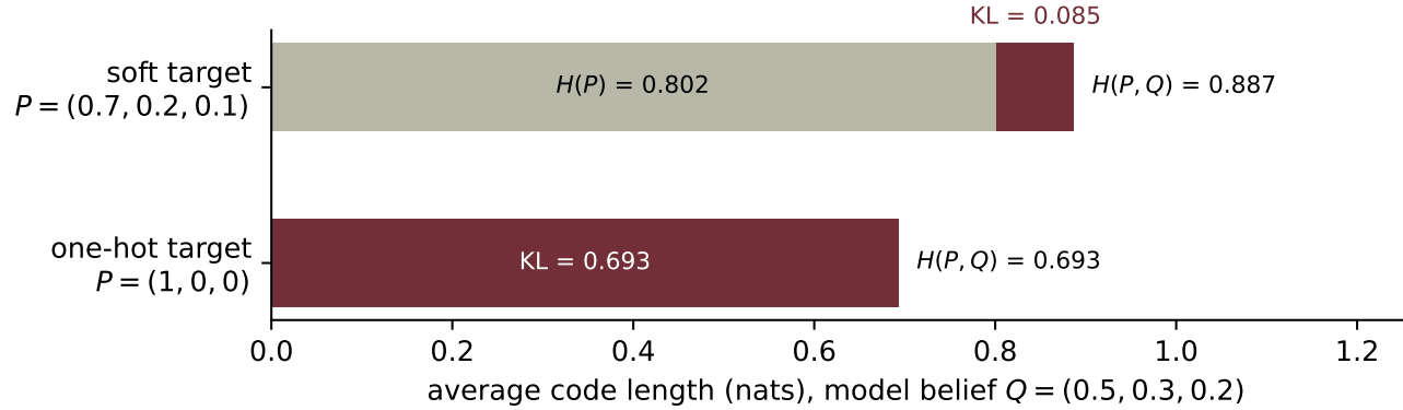
Figure 2.4.: Cross-entropy splits into the target’s own entropy plus the KL divergence, the extra code length paid for using the model’s belief Q . The model belief is the same in both rows. A soft target (top) carries entropy of its own; a one-hot target (bottom) carries none, so its whole cross-entropy is KL divergence, the surprise -\log q_{\text{true}} .
