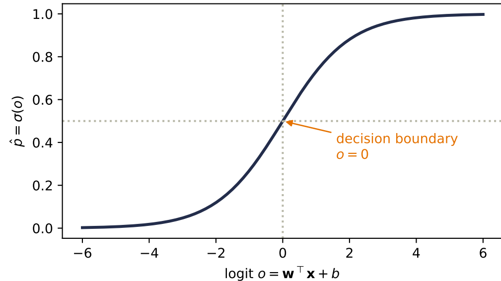
score to probability
