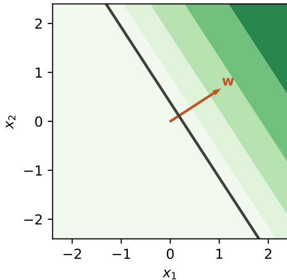
the threshold in input space
