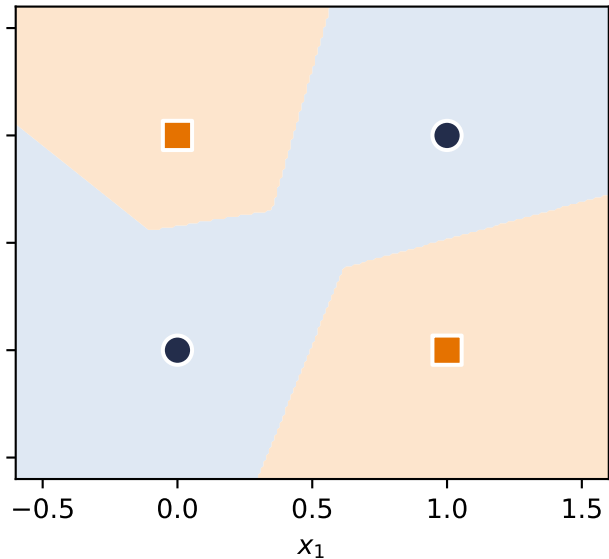
trained MLP (100%)
