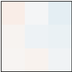
random start
