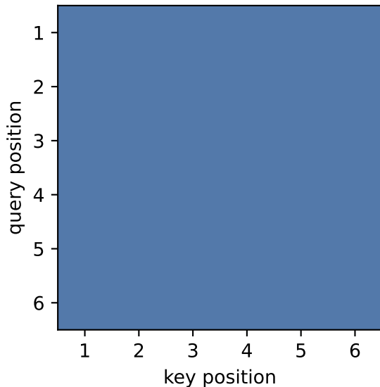
BERT-style encoder
