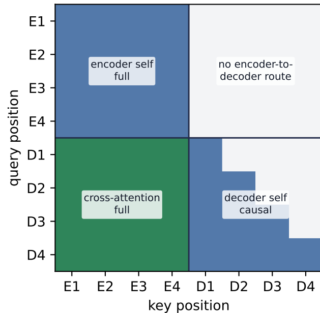
T5-style encoder-decoder
