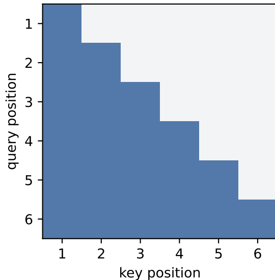
GPT-style decoder
