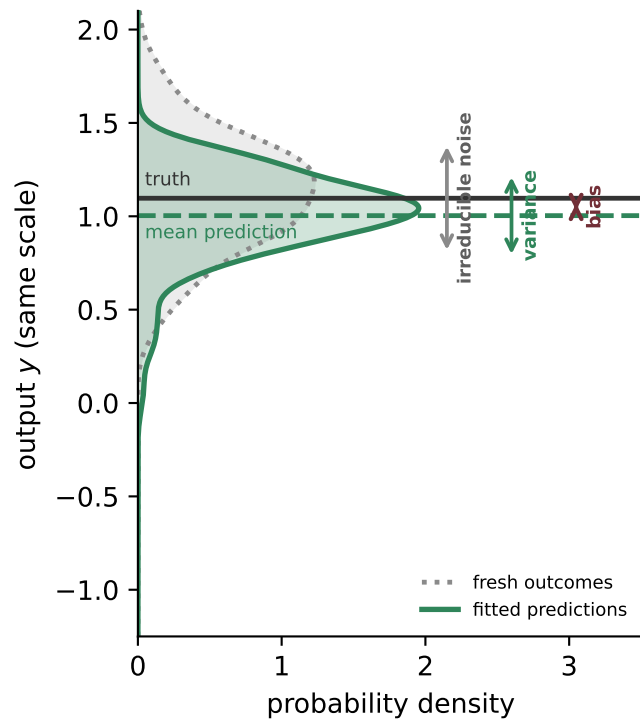
B Slice at x_0 = 0.65
