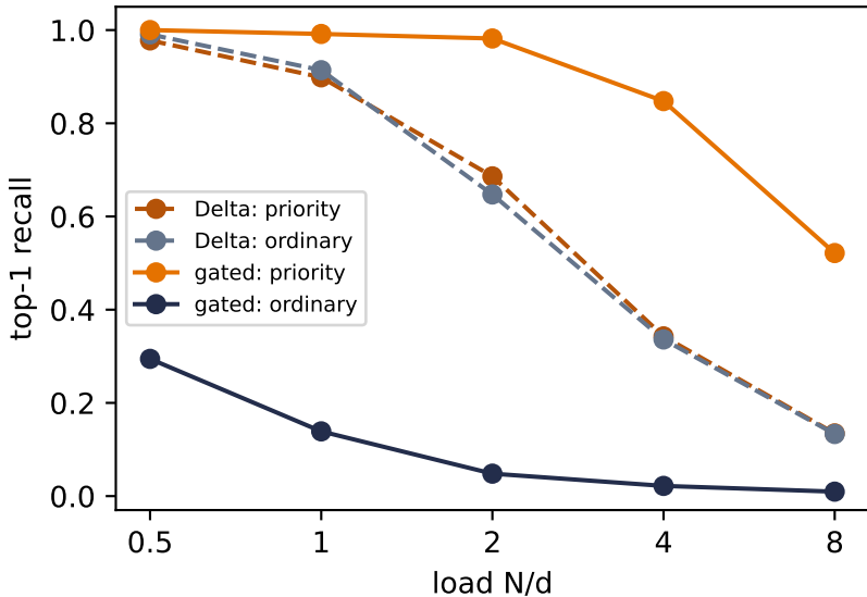
Gated delta update
