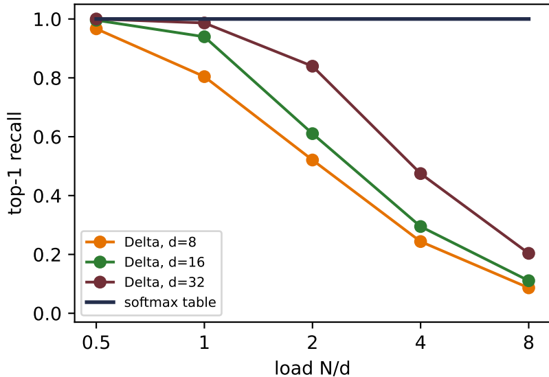
One-pass delta update with a fixed state
