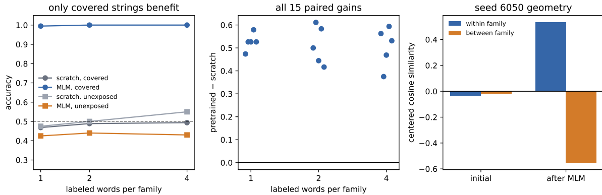
Figure 15.4.: Five paired end-to-end seeds in the synthetic transfer lab. MLM initialization separates covered latent families and improves every covered-type comparison (left and center); both arms stay near chance on input-vocabulary controls withheld from MLM inputs, replacements, and targets (left). Centered cosine similarity is a representation diagnostic, not a task metric (right).
