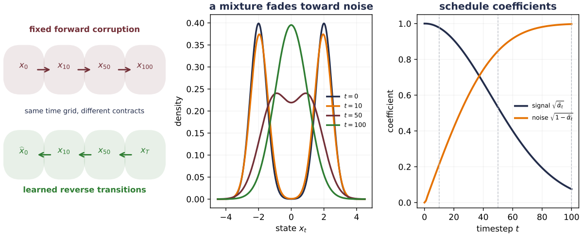
Figure 19.6.: Forward diffusion replaces a two-mode distribution by an almost standard-normal endpoint. Under the displayed 100-step schedule, \alpha -bar is 0.954508 at t = 10 , 0.282981 at t = 50 , and 0.005619 at t = 100 . The final signal and noise coefficients are 0.074958 and 0.997187. The lower chain is learned in the opposite direction; it is not the algebraic inverse of one realized forward chain.
