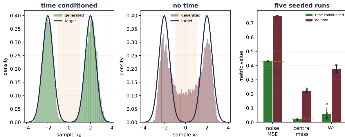
Figure 19.7.: A designed one-dimensional diffusion sampler isolates the value of time conditioning. Across seeds 6050–6054, the time-conditioned denoiser has evaluation noise MSE 0.429707 (SD 0.000927), close to the analytic conditional-mean oracle’s fixed-evaluation MSE of 0.425920. Its generated samples have mean standard deviation 2.062095, central mass 0.019470, and Wasserstein-1 distance 0.058570 from a matched target sample; the population targets are 2.061553 and 0.022750 for standard deviation and central mass. Removing t raises noise MSE to 0.750634, central mass to 0.222760, and Wasserstein distance to 0.375321. This is a CPU mechanism study of a planted scalar mixture, not an image-generation result.
