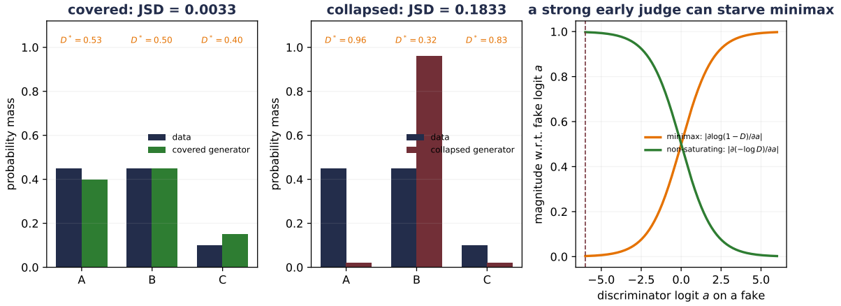
Figure 19.5.: A finite three-mode GAN audit. The covered generator q = (0.40, 0.45, 0.15) has Jensen–Shannon divergence 0.003253 and optimal-discriminator value -1.379789 . The collapsed q = (0.02, 0.96, 0.02) has divergence 0.183270 and value -1.019755 ; both satisfy V(D^*, G) = -\log 4 + 2 \text{ JSD} to floating-point precision. When the discriminator assigns a fake logit -6 , its output is 0.002473 : the original minimax generator’s logit-gradient magnitude is 0.002473 , versus 0.997527 for the non-saturating loss.
