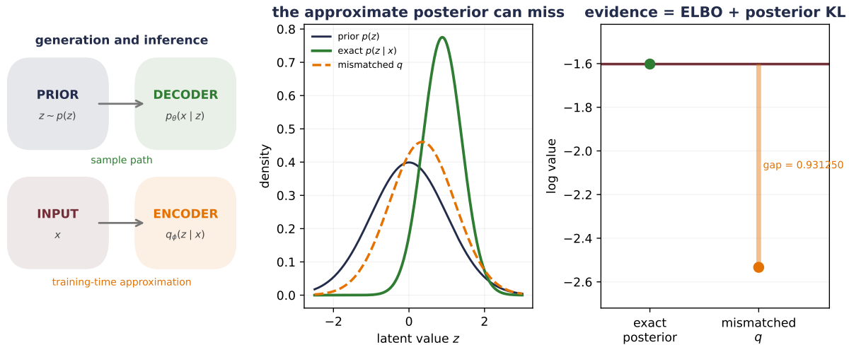
Figure 19.4.: The VAE lower bound is audited in a one-dimensional Gaussian model. For x = 1.2 and observation variance 0.36, the exact posterior has mean 0.882353 and variance 0.264706. The log evidence and exact-posterior ELBO are both -1.602093. For q = N(0.35, 0.75) , the ELBO is -2.533343; its 0.931250 gap to the evidence exactly matches KL(q \parallel p(z \mid x)) .
