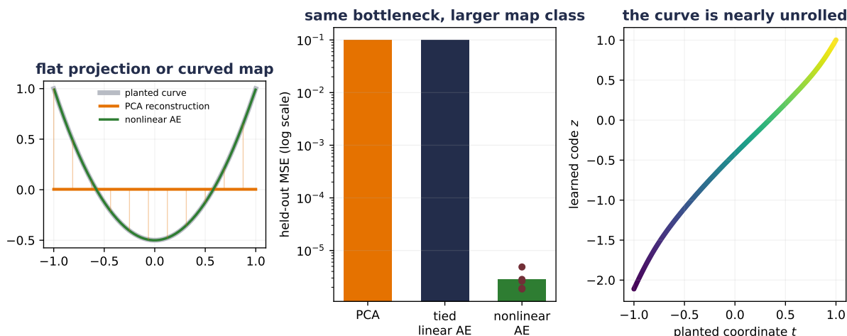
Figure 19.2.: A one-dimensional bottleneck behaves differently when its maps may bend. On the alternating held-out grid, rank-one PCA and the tied linear autoencoder both have MSE 0.100000 and their projectors agree to displayed precision. Across seeds 6050–6054, the nonlinear autoencoder has mean held-out MSE 0.000002815 (SD 0.000001223); the absolute Pearson correlation between its code and the planted coordinate has mean 0.992802 (SD 0.005513). This controlled curve and capacity-mismatched model show a mechanism, not a universal nonlinear-autoencoder advantage.
