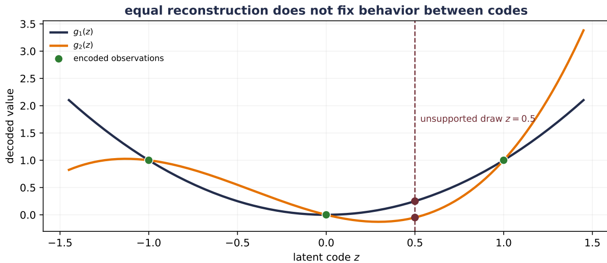
Figure 19.3.: Reconstruction does not identify a latent sampler or a unique decoder away from observed codes. The two displayed decoders agree exactly at z equal to -1, 0, and 1, so both have zero reconstruction error on the three targets. They disagree between and beyond those codes; at z = 0.5 their outputs are 0.25 and -0.05.
