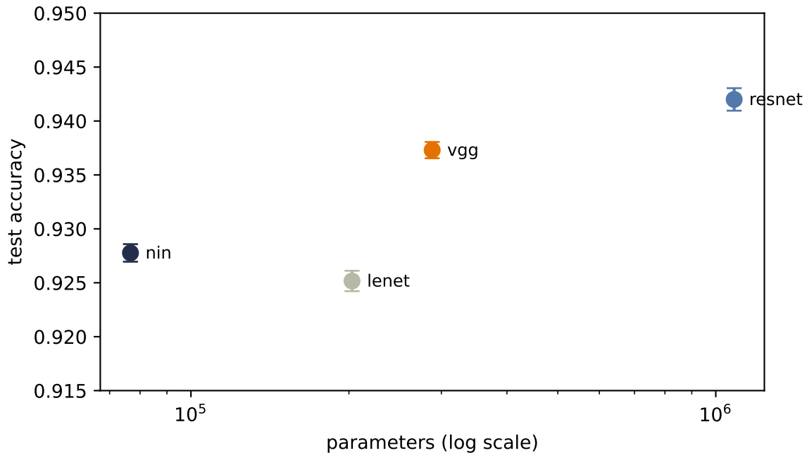
Figure 9.5.: The full-data Part II scorecard on Rivanna. Points show mean official-test accuracy and bars one sample standard deviation across seeds 6050–6052. LeNet reaches 92.52%, NiN 92.78%, VGG 93.73%, and the residual network 94.20%. NiN is the most parameter-efficient point; VGG buys more accuracy with depth; residual blocks reach the strongest endpoint in this declared training regime. Parameter count is not training compute, and these four points are not a universal architecture ranking.
