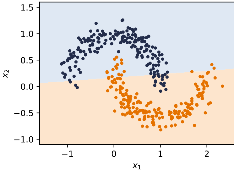
linear: 89.7%
