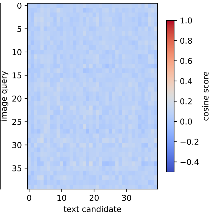
shuffled · seed 6052
