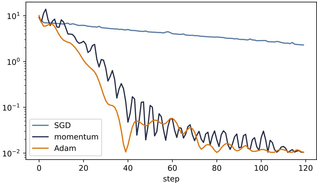
full-batch loss (log scale)
