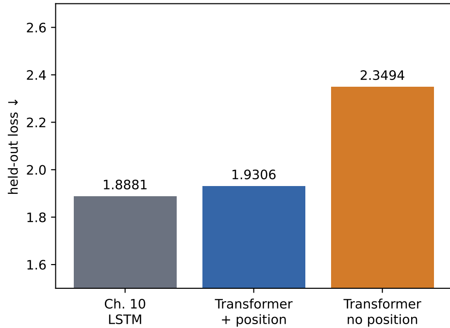
fixed-window rematch
