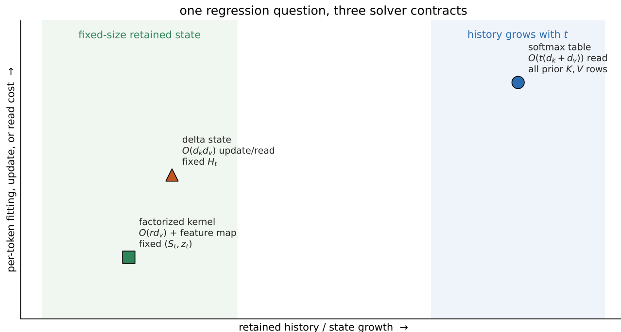
Figure TTR.1: The solver map compares retained state and per-token work. Its positions are qualitative; the formulas and direct labels carry the exact ledger.
