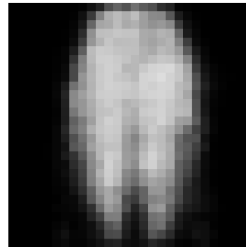
denoising AE
