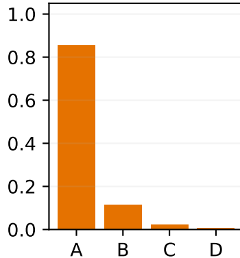
softmax, \tau = 0.5
