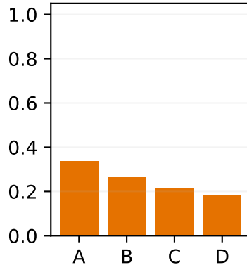
softmax, \tau = 4
