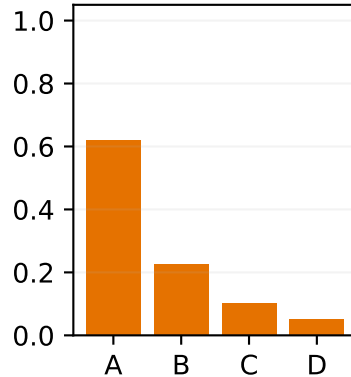
softmax, \tau = 1
