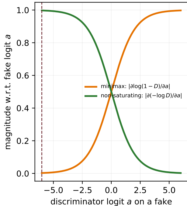
a strong early judge can starve minimax
