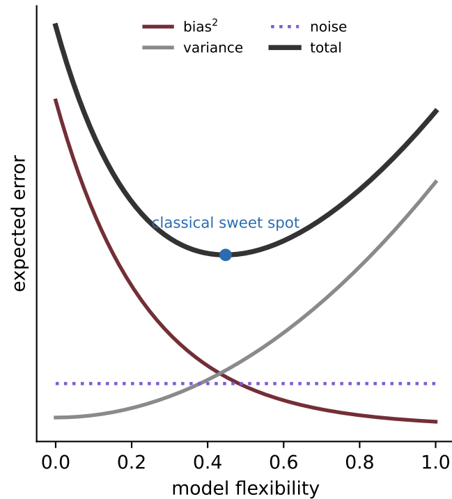
C Classical summary
