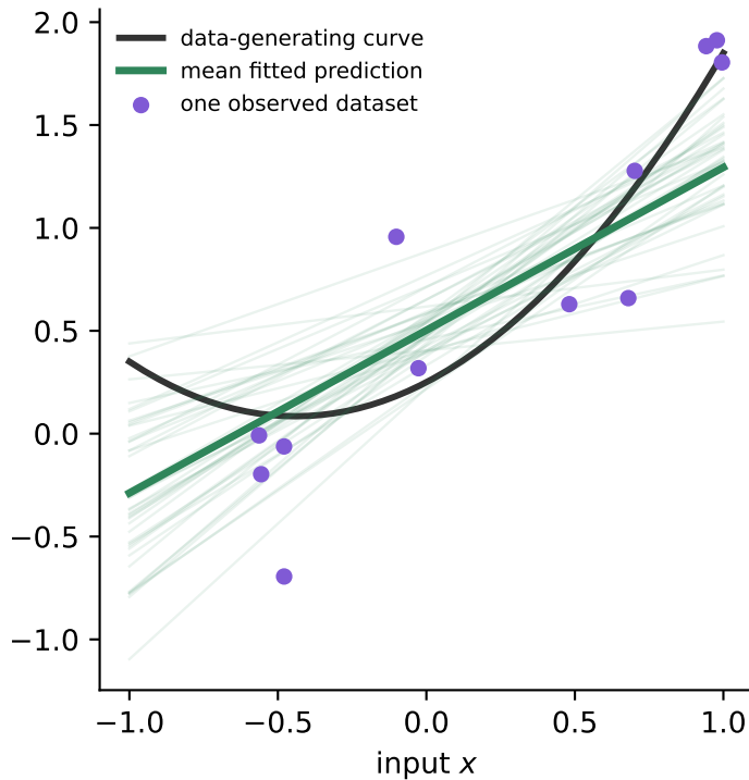
A Fresh data, fresh fit
