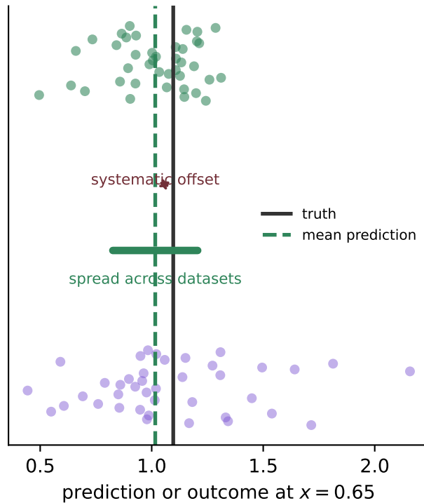
B Hold the input fixed
