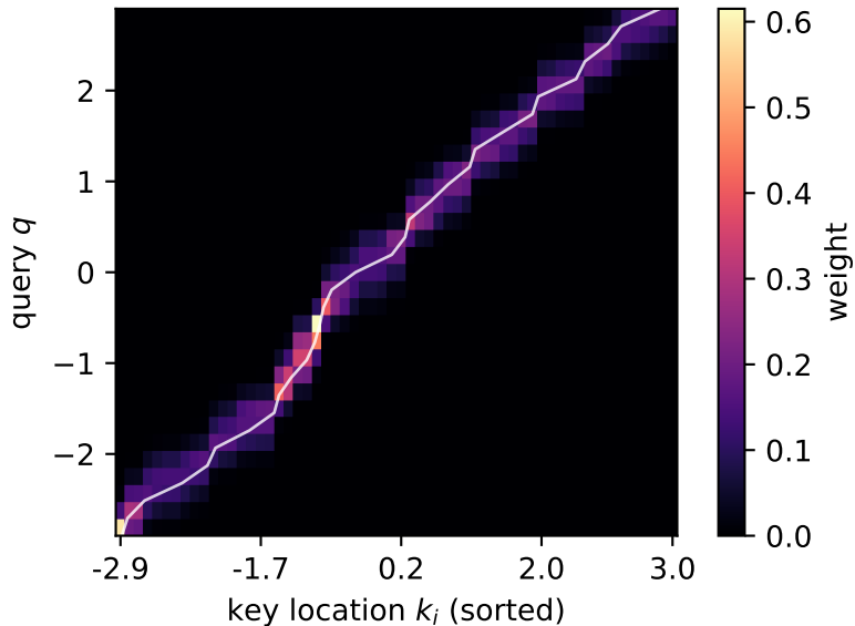
Fixed attention matrix, h = 0.18
